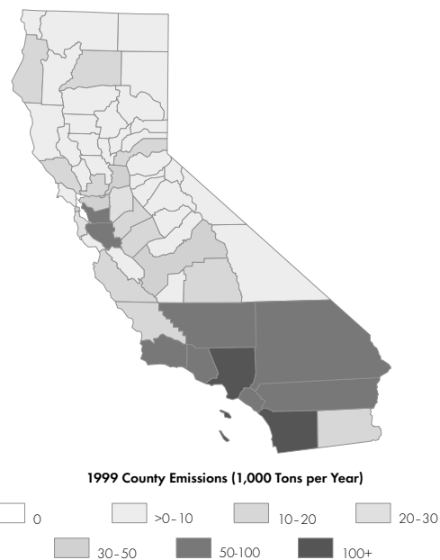
FIGURE 9 California NO x Emissions
